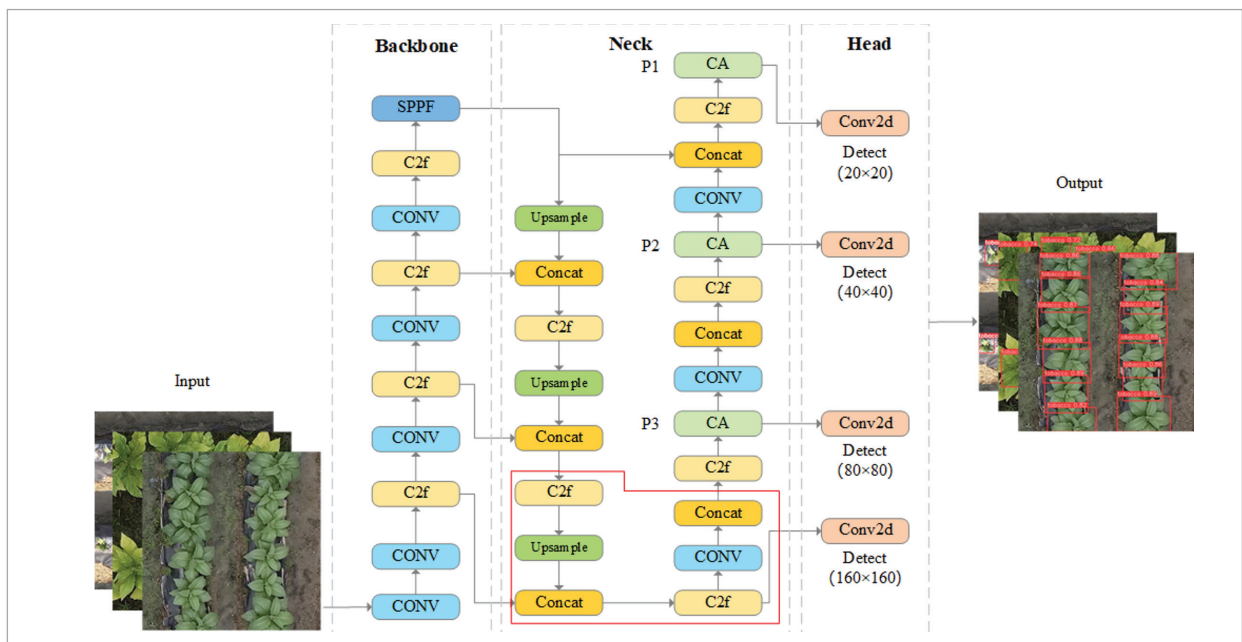
Network Structure Diagram of YOLOv8-CSD Model.
