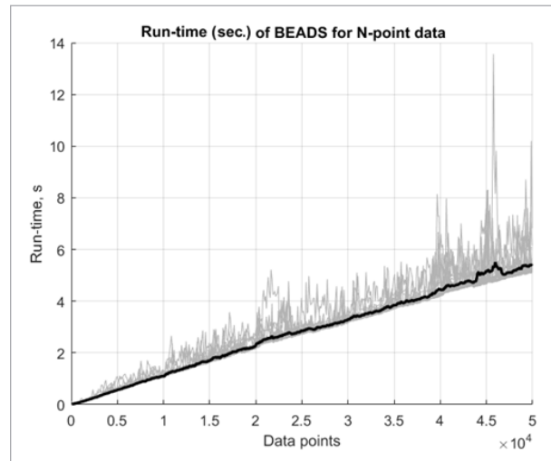
Figure 6 Complexity of BEADS algorithm
