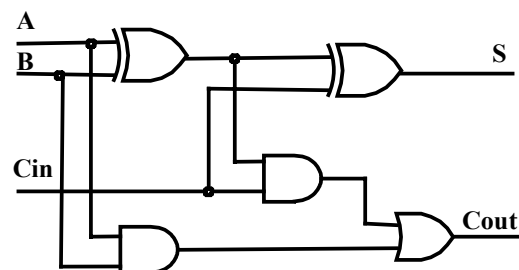
Figure 4. Schematics of naive 1-bit adder implementation
