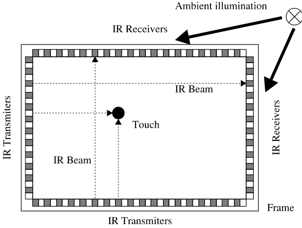
Figure 1. Arrangement of optical IR transmitters and receivers within the Touch interface
