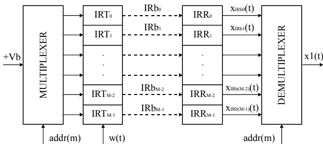
Figure 2. Functional block diagram of Touch interface
