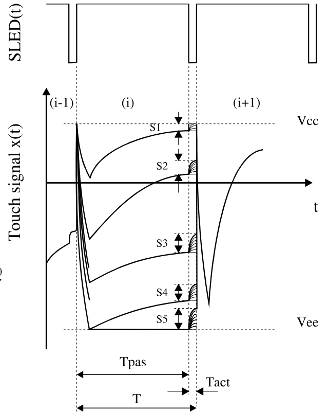
Figure 3. Touch signal in the period of activity of the i -th optical pair
