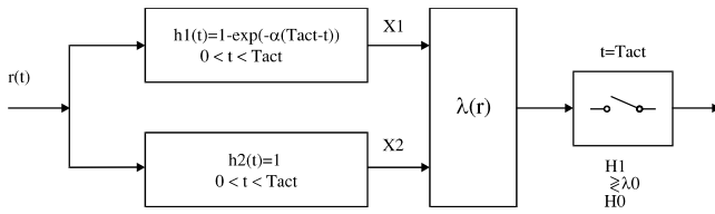
Figure 5. Optimal receiver
