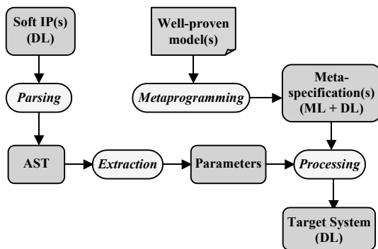
Figure 5. Design flow in Model 3
