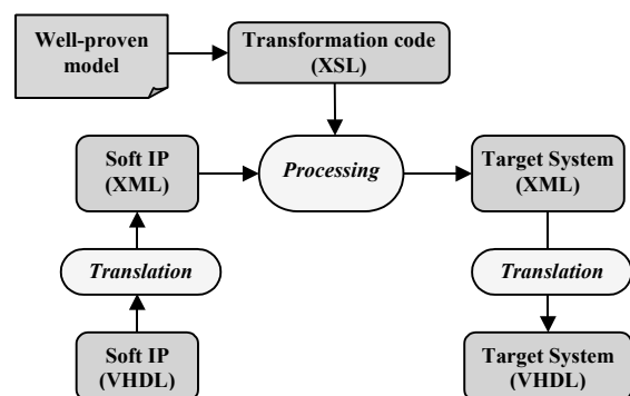
Figure 6. Design flow in Model 4
