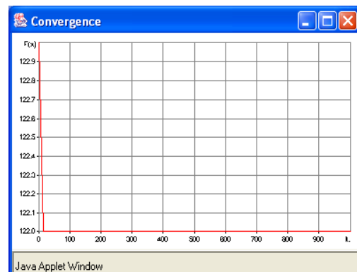
Figure 16. Variation of variable when the number of iteration is growing in “Mig1” method
