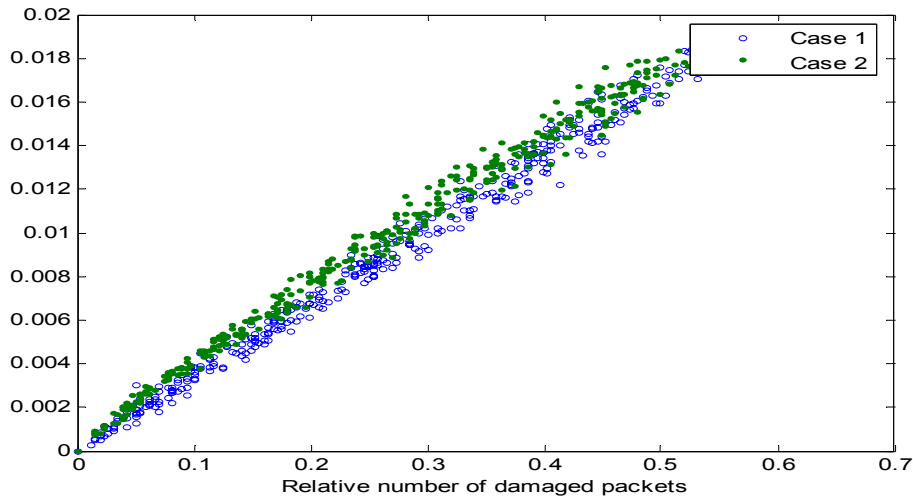
Figure 12. DAD degradation factor for two NCS configurations: Case 1 – circles and Case 2 – dots of a closed loop control system with packets loss vs. the relative number of lost packets. DAD also gives best results. Unfortunately, it requires computation of two approximated SVD-DFT diagrams for NCS and non-NCS case. If the nominal model is known, DAD is probably the best degradation degree out of the four introduced in this paper
