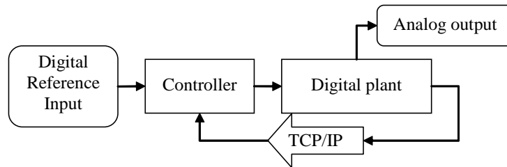
Figure 6. NCS with a remote sensor. Simplified network configuration is used when the measure is transmitted over the network channel and the actuator is available directly at the controller
