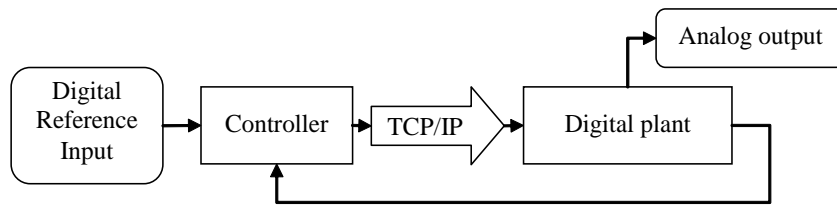
Figure 5. NCS with a remote actuator. Simplified network configuration is mainly used when the measure is available in the controller, however the actuator is situated at a relatively long distance
