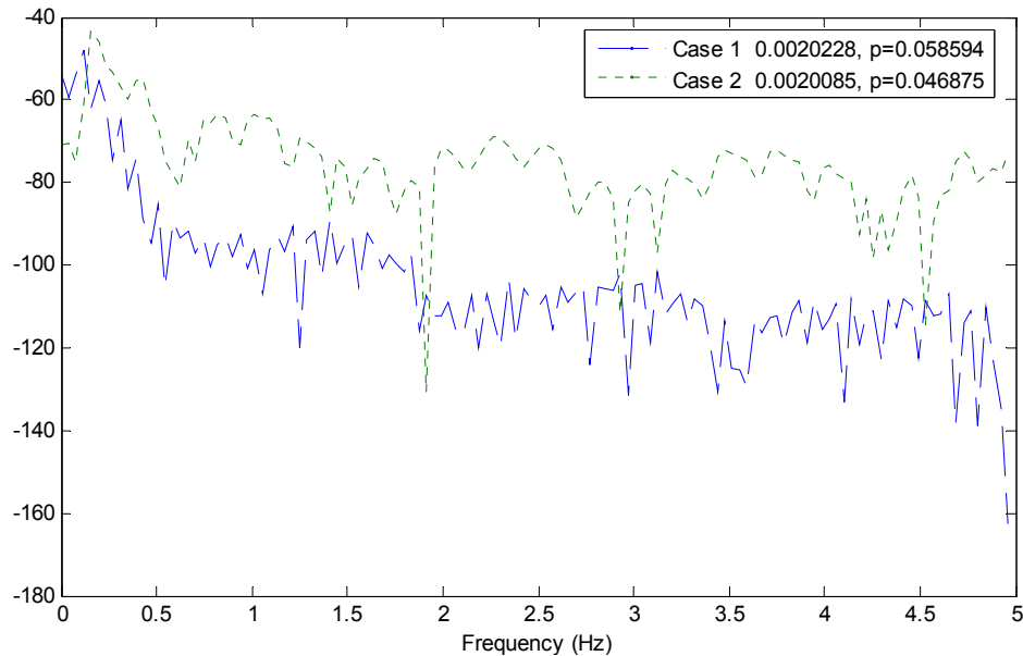
Figure 14. Difference between transformed impulse responses (magnitude only) for NCS with similar degradation factors: Case 1 – solid line, Case 2 – dotted line. Similar level of DD results in the similar range of the frequency error. High frequency disturbances which are visible in the step response in case 2 correspond to higher levels of the difference frequency response for high frequencies. Nevertheless error for low frequencies is larger in case 1 which is due to similar levels of DAD
