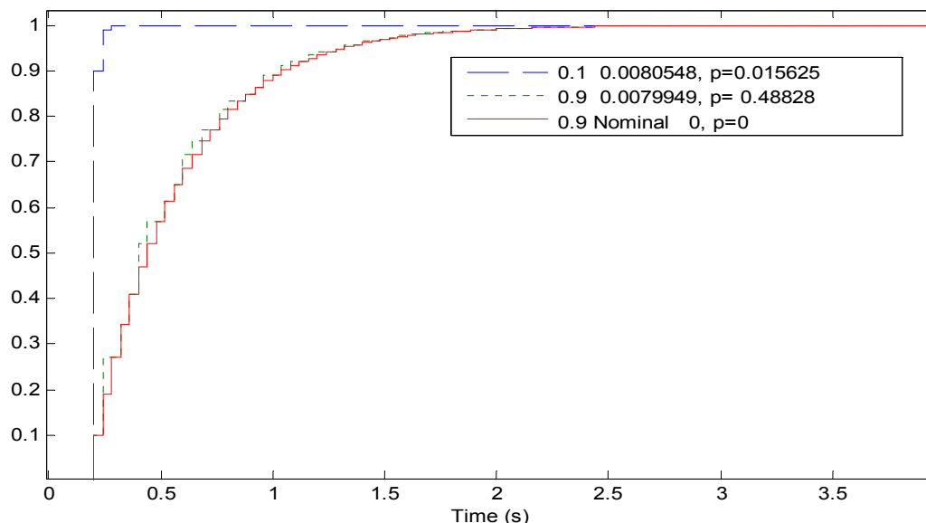
Figure 10. Step responses for fast (solid line) and slow (dotted line) time lag systems with packet delays. The degradation of the step responses for approximately the same WRD are rather similar however the definitions are based on the frequency domain, and the differences in the time domain do not need to correspond to the computed degradation degree
