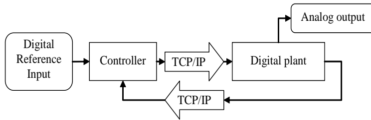
Figure 4. NCS with a remote controller and remote plant. The configuration is the most often used for remote monitoring and control. It consists of two unidirectional or one bidirectional network channels
