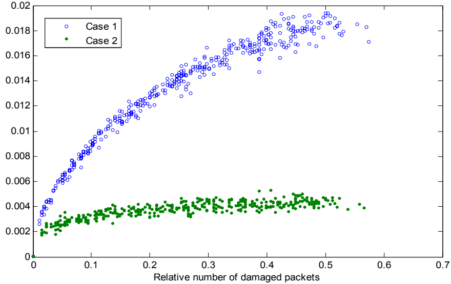
Figure 11. WBA degradation factor for two NCS configurations: Case 1 – circles and Case 2 – dots of a closed loop control system with packets loss vs. the relative number of lost packets. The definition gives concentrated results however the WBA is less linear than DAD
