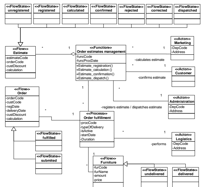
Figure 5. Generated Class model for the management function “Order estimates management”
