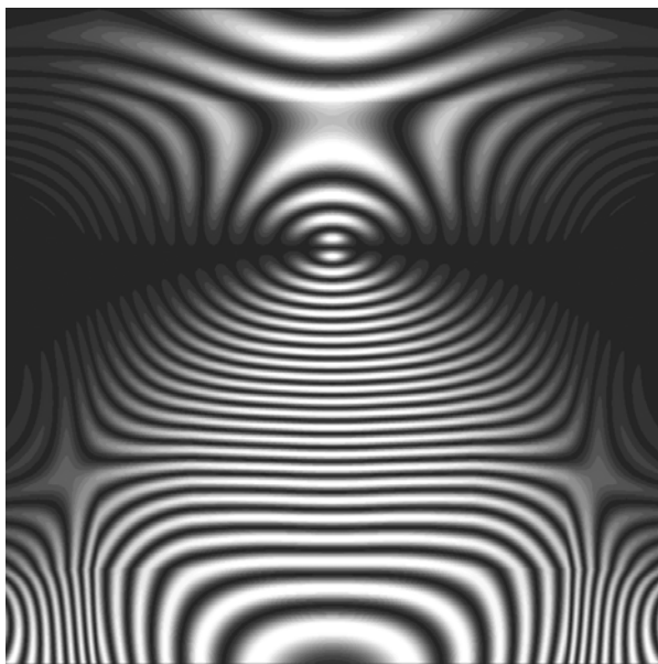
Figure 6. Isoclinics and isochromatics intertwined for the third eigenmode at \alpha = 0
