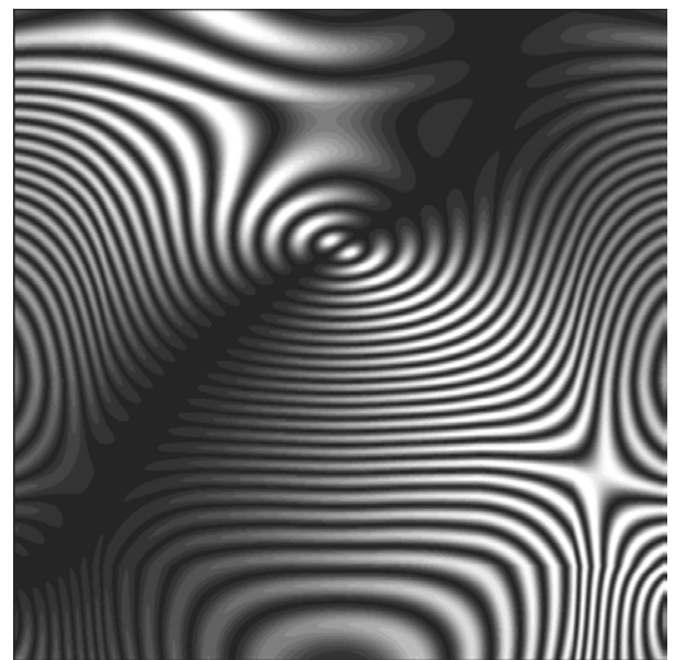
Figure 8. Isoclinics and isochromatics intertwined for the third eigenmode at \alpha = \pi/8
