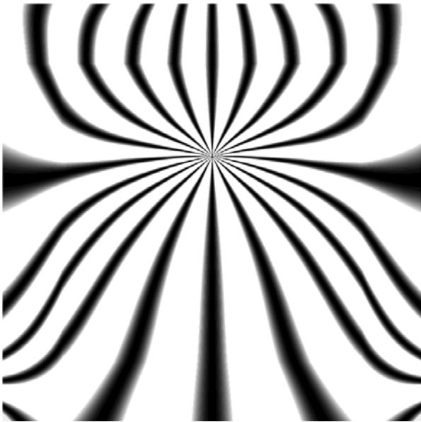
Figure 9. The lines of the principal direction of the stresses for the third eigenmode at \alpha = (i-1)\pi/20 , i = 1, \dots, 10
