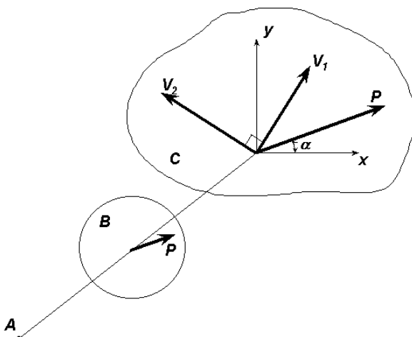
Figure 1. The schematic structure of a plane polariscope: A – the light source; B – polarizer (analyser is not shown); C – stressed specimen; x, y – axes of the orthogonal Cartesian frame; \{P\} - the vector of polarisation; \{V_1\}, \{V_2\} - the directions of the principle stresses.
