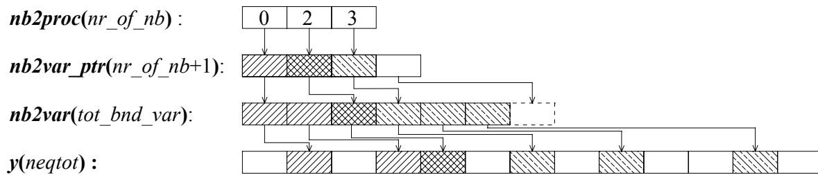
Figure 1. Data structures for inter-processor communication
